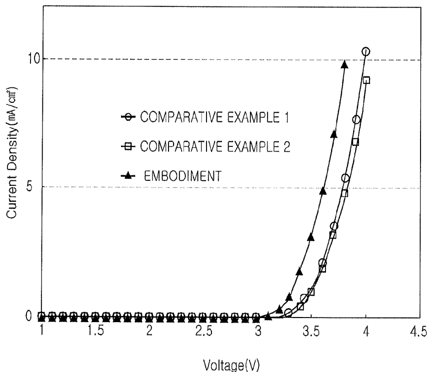
I-V Curve
